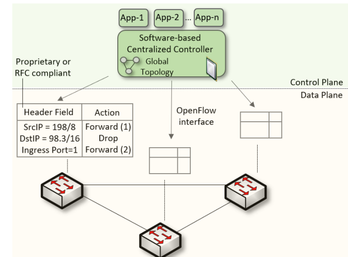
SDN network
